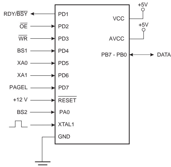
Figure 127. Parallel Programming
